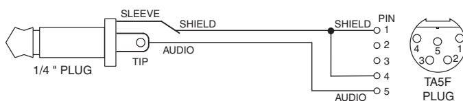
Wiring diagram
